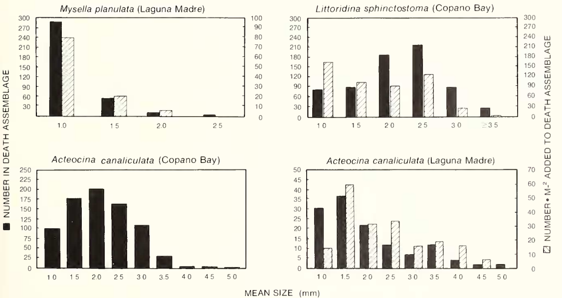
TEXT-FIG. 7. Comparison of the average size-frequency distribution in the death assemblage and the calculated size-frequency distribution of living individuals that died during the study period for miscellaneous taxa. Number in the death assemblage is the total number actually collected during the study.
